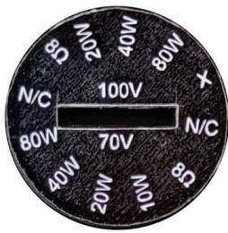
Power taps
